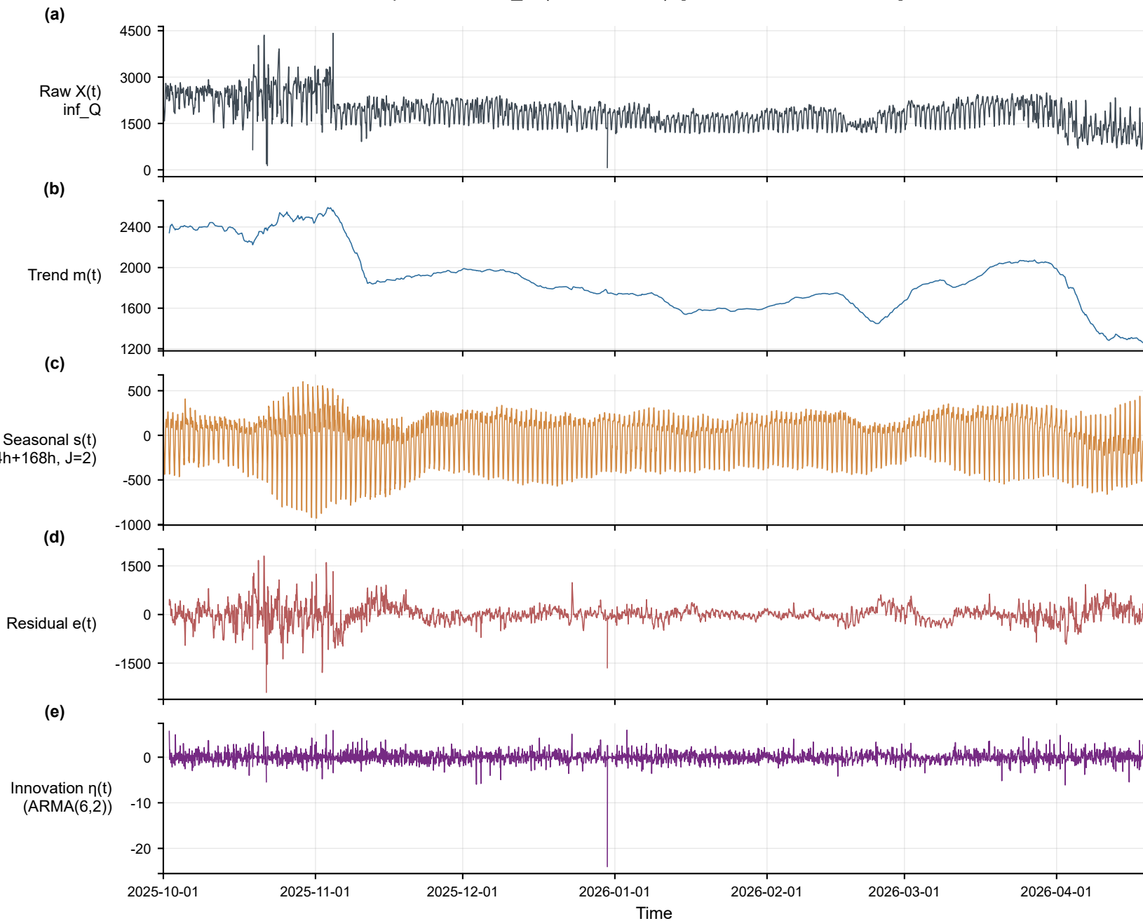
Multi-scale decomposition — inf_Q (influent, hour) [2025-10-01~2026-04-19]
